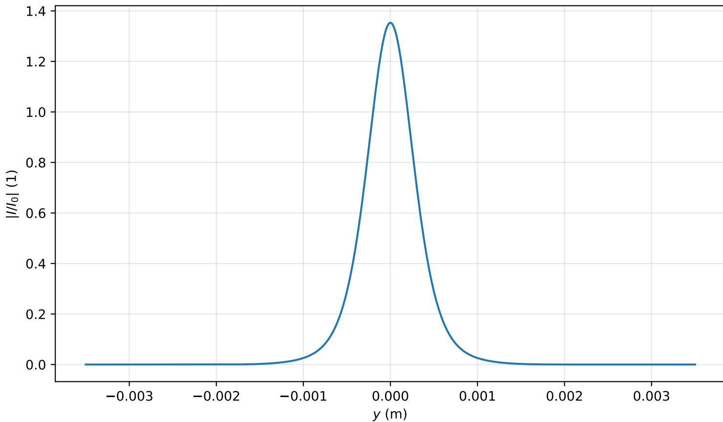
Intensity profile I(x=0, y, z=1.672)/I_0 , P_{in}=0.8P_{cr} , artificial time
